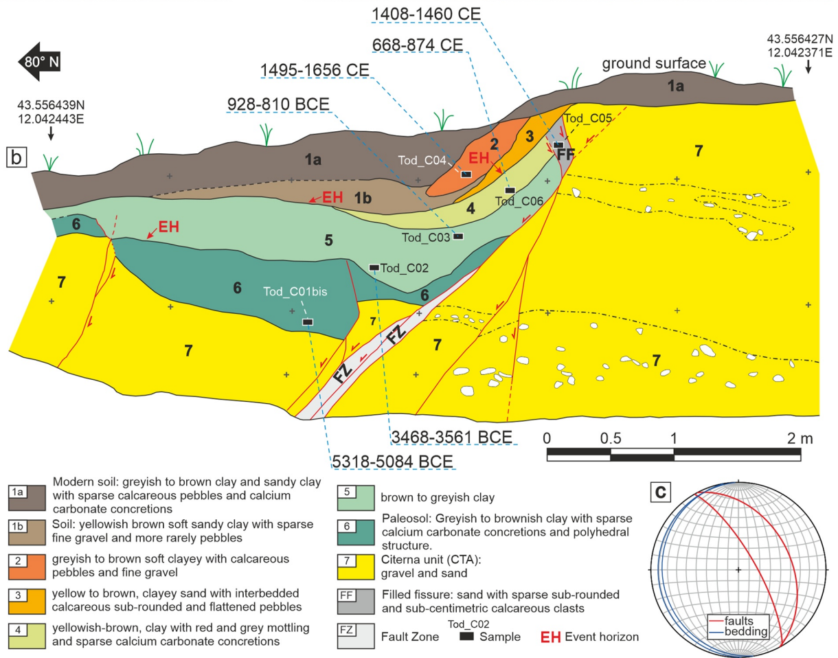
Figure 9. (a) Detailed view of the Todari roadcut; (b) interpretation of the Todari roadcut, with the age of the samples; (c) the attitude of the fault and bedding are shown in the stereo plot.
